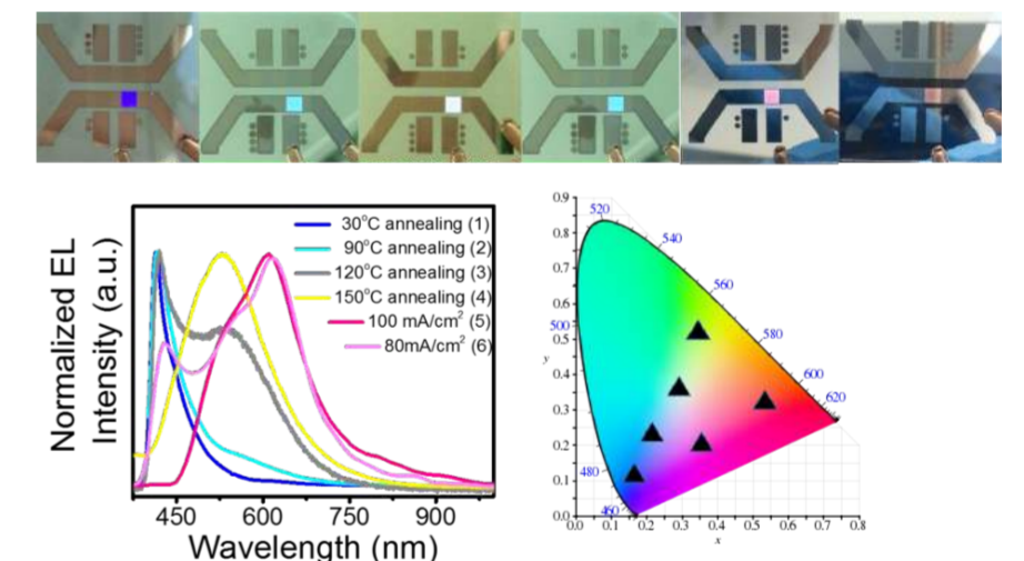
有机小分子 TPEPA 在不同温度下产生荧光改变及不同色温的 OLED 器件 OLED device with organic small molecule TPEPA as emissive layer that produces light covering nearly whole visible spectra controlled by different temperatures
